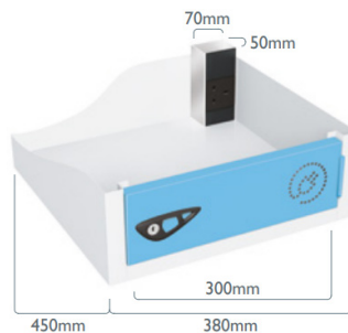
Pure Laptop Charging Lockers - 15 Door - 15 Compartment
